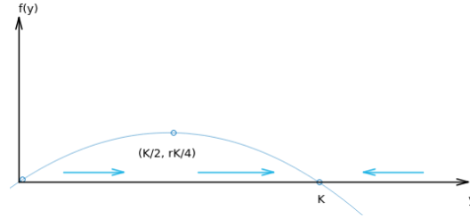
Figure 4.7: The equilibrium solution f(y) = 0 or r(1 - y/K)y = 0 to visualize other solutions of Eq. (4.53) ( Hamzstplot/Examples with Makefile/Plot 2D Equilibrium Solution for Logistic Growth/main.cpp ).
