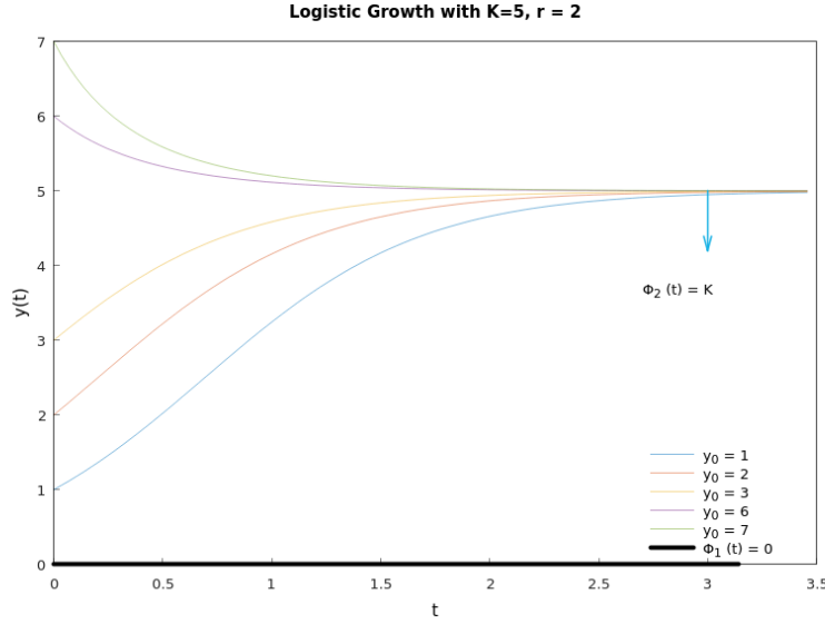
Figure 4.8: The solution curves for y(t) = \frac{y_0 K}{y_0 + (K - y_0)e^{-rt}} to visualize all possible solutions of Eq. (4.53) with different y_0 (Hamzstplot/Examples with Makefile/Plot 2D Solution Curves for Logistic Growth/main.cpp).
