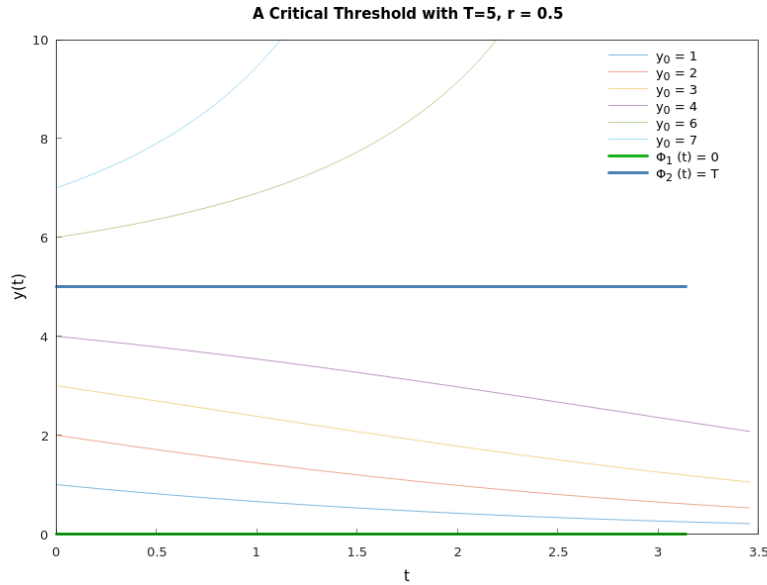
Figure 4.11: The solution curves for growth with a threshold for \frac{dy}{dt} = -r \left(1 - \frac{y}{T}\right) y (Hamzstplot/Examples with Makefile/Plot 2D Solution Curves for Critical Threshold/main.cpp).
